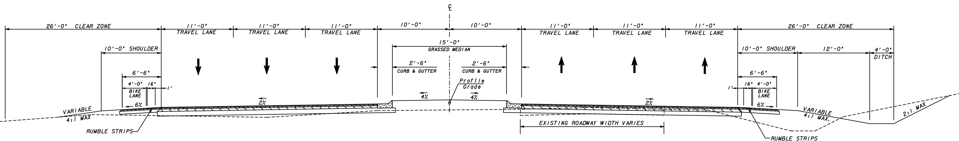
TYPICAL SECTION (FROM MALONE ROAD TO BILL CARRUTH PARKWAY)
